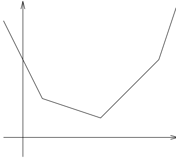
Figure 1.2: A convex piecewise linear function.
