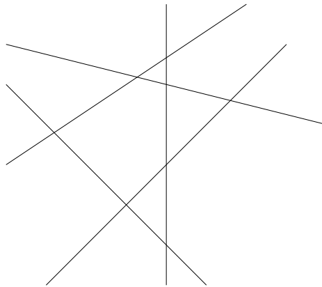
Figure 1.1: An arrangement of lines.
