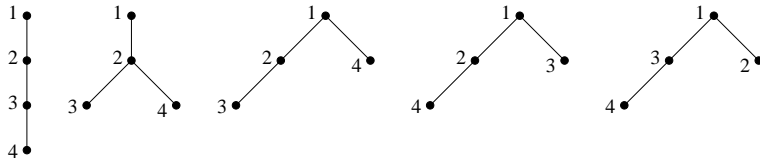
Figure 4: The five increasing (1,2) -trees with four vertices
