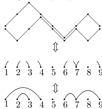
Figure 2.2: A pair of noncrossing free Dyck paths and its corresponding partition.
