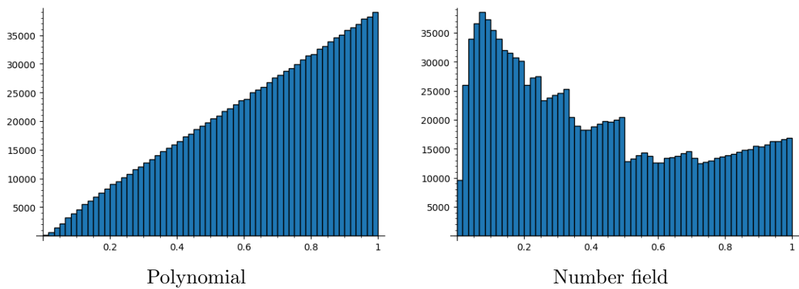
Figure 6: Normalized root discriminants for g = 2 .
