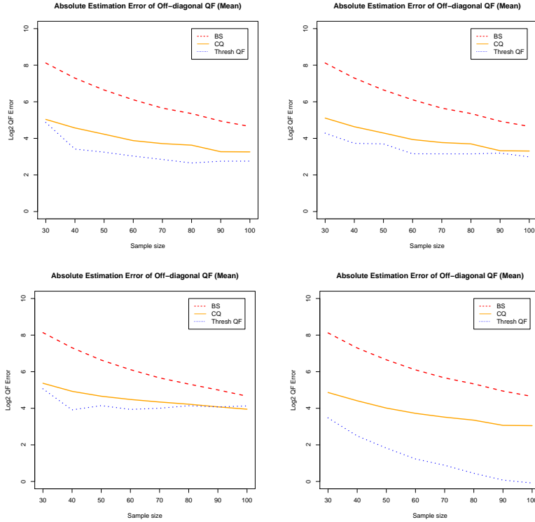
Fig 2: Performance of estimating Q(\Sigma) using thresholded estimator \hat{Q} (blue dotted), CQ-\hat{D} (orange solid) and BS-\hat{D} (red dashed). The mean of absolute errors over 500 repetitions in log scale (base 2) versus the sample size were reported for matrix M1 (top left), M2 (top right), M3 (bottom left), M4 (bottom right).
