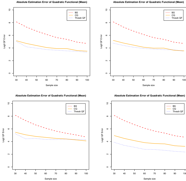
Fig 1: Performance of estimating \|\Sigma\|_F^2 using thresholded estimator \hat{Q} + \hat{D} (blue dotted), CQ (orange solid) and BS (red dashed). The mean of absolute errors over 500 repetitions in log scale (base 2) versus the sample size were reported for matrix M1 (top left), M2 (top right), M3 (bottom left), M4 (bottom right).
