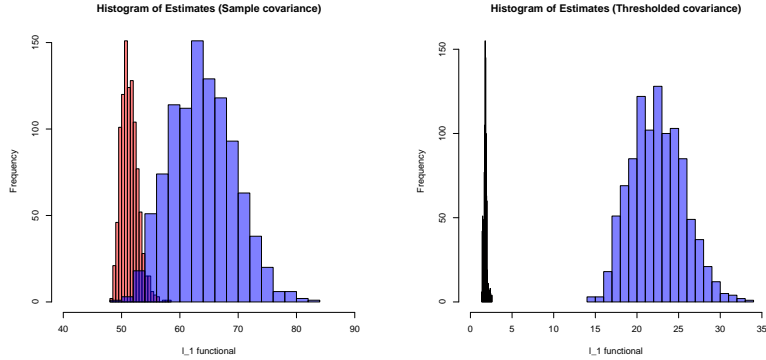
Fig 3: Histogram of 1000 \ell_1 functional estimates for H_0 (red) and H_1 (blue) by \ell_r(\hat{\Sigma}) (left) and optimal estimator \ell_r(\tilde{\Sigma}_\tau) (right).
