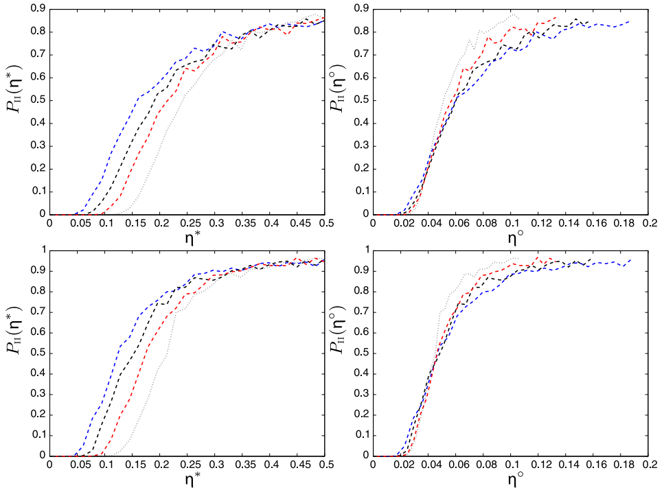
FIG. 2. Probability of type II error P_{\text{II}}(\eta) with scalings \eta = \eta^* (left) and \eta = \eta^\circ (right) for p = \{50, 100, 200, 500\} , k = \lfloor \sqrt{p} \rfloor , N = 1400 . Test levels are \alpha = 5\% (top) and \alpha = 1\% (bottom).
