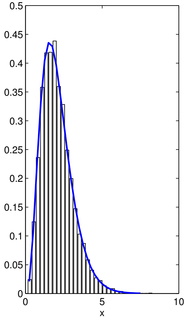
pdf of \lambda_{\min} of 5 \times 5 6-Laguerre, a=16
