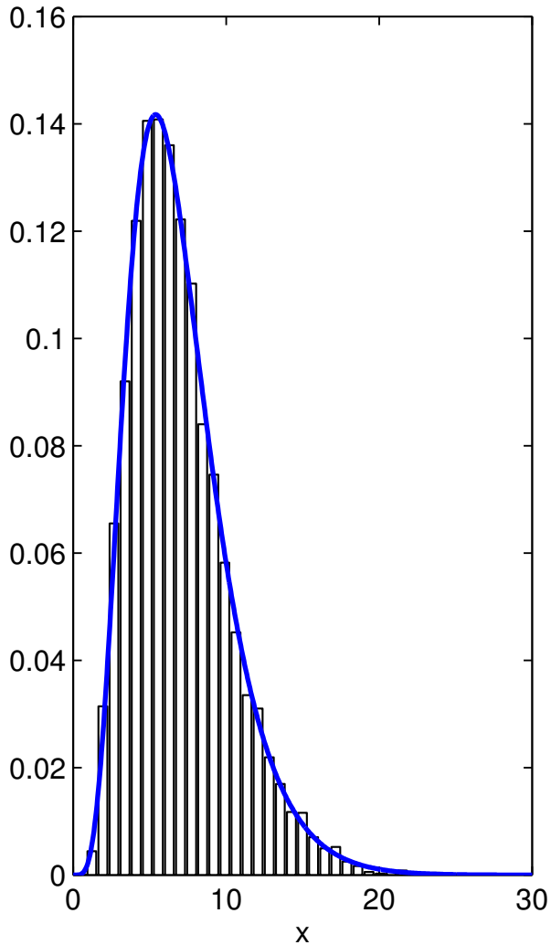
pdf of \text{tr}(A) , A=W_3(4,\text{diag}(0.25,0.5,1))
