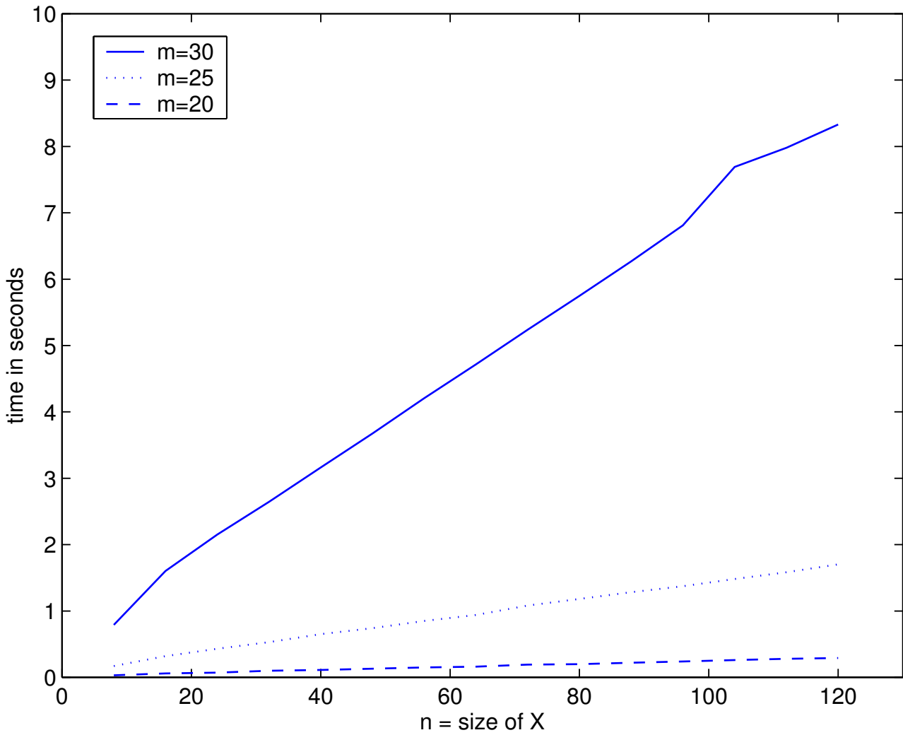
Time to compute {}_0^m F_0^{(2)}(X)
