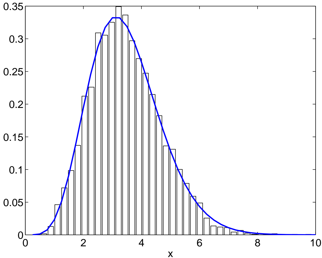
pdf of \lambda_{\min} of (9 \times 9) Wishart with L=20 degrees of freedom
