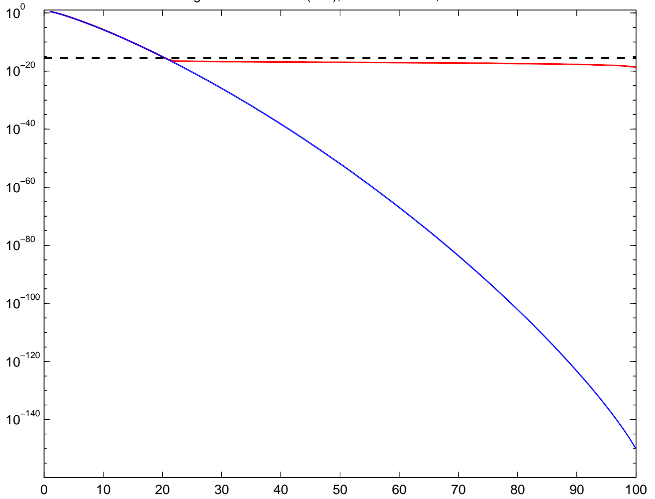
Singular values of Hilb(100), blue = accurate, red = usual
