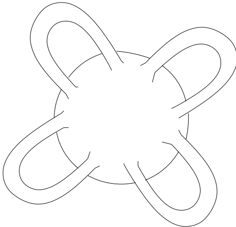
FIGURE 1. A handlebody of genus 4.
