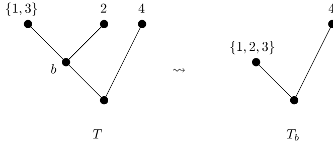
Figure 3-11: An example of bud collapse for generalized \{1, 2, 3, 4\} -labelled trees
