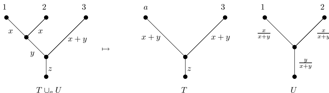
Figure 3-8: The map \bar{w}(T \cup_a U) \rightarrow \bar{w}(T) \wedge \bar{w}(U)
