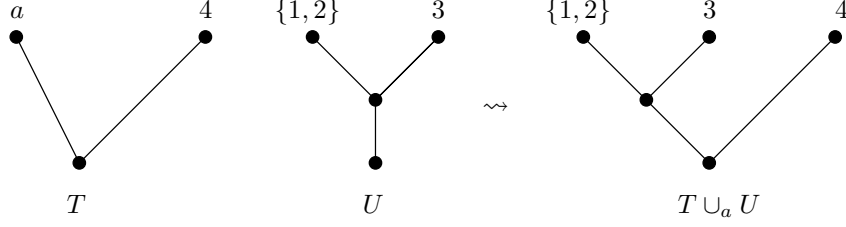
Figure 3-13: Grafting generalized labelled trees
