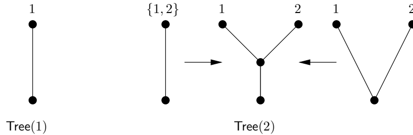
Figure 3-12: Tree(1) and Tree(2) (the arrows represent the direction of the morphisms in Tree(2))
