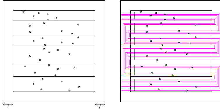
Figure 7-2: Left: The grid H , the points in S'' , and their grouping. Here \ell = 6 . Right: Construction of the minor \ell \times \ell grid R passing through the points in S'' .
