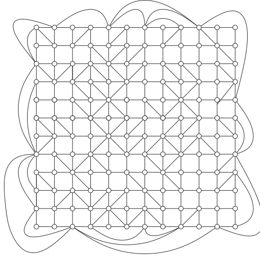
Figure 4-1: A partially triangulated (12 \times 12) -grid.
