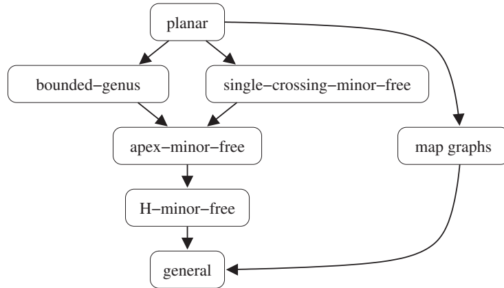
Figure 1-1: Interesting classes of graphs. Arrows point from more specific classes to more inclusive classes.
