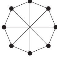
Figure 2-2: The graph V_8 .
