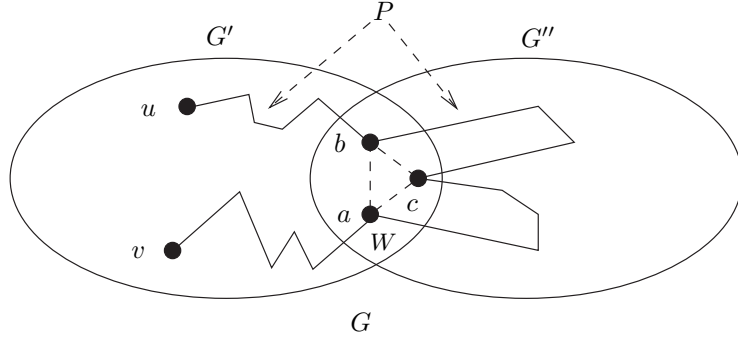
Figure 2-3: The replacement of the part of path P between a and b by edge \{a, b\} .
