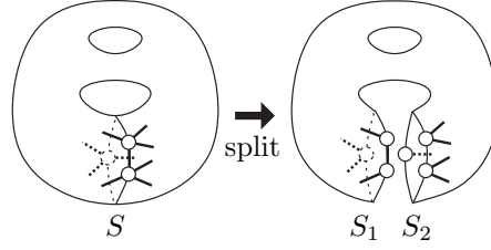
Figure 5-1: Splitting a noose.
