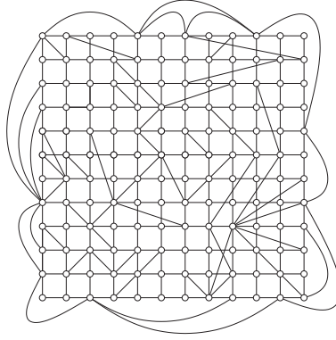
Figure 7-1: An augmented 12 \times 12 grid with span 8.
