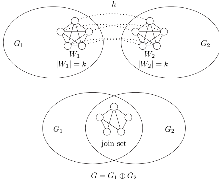
Figure 1-2: Example of a 5-sum of two graphs.
