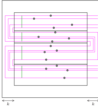
Figure 6-1: Construction of the minor k \times k grid K .
