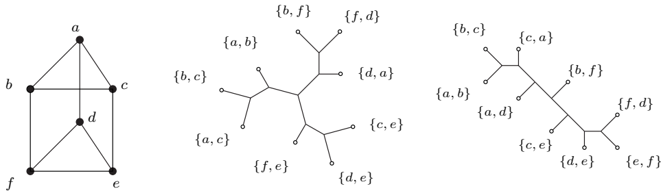
Figure 2-4: A graph and two branch decompositions of it. The first has width 4 and the second has width 3.
