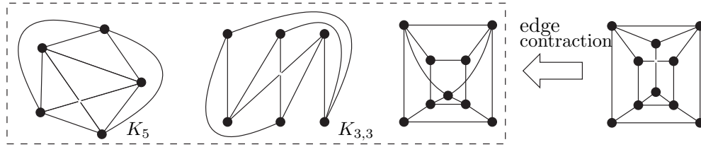
Figure 2-1: Examples of single-crossing graphs
