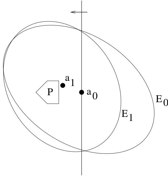
Figure 7.1: One iteration of the ellipsoid algorithm.
