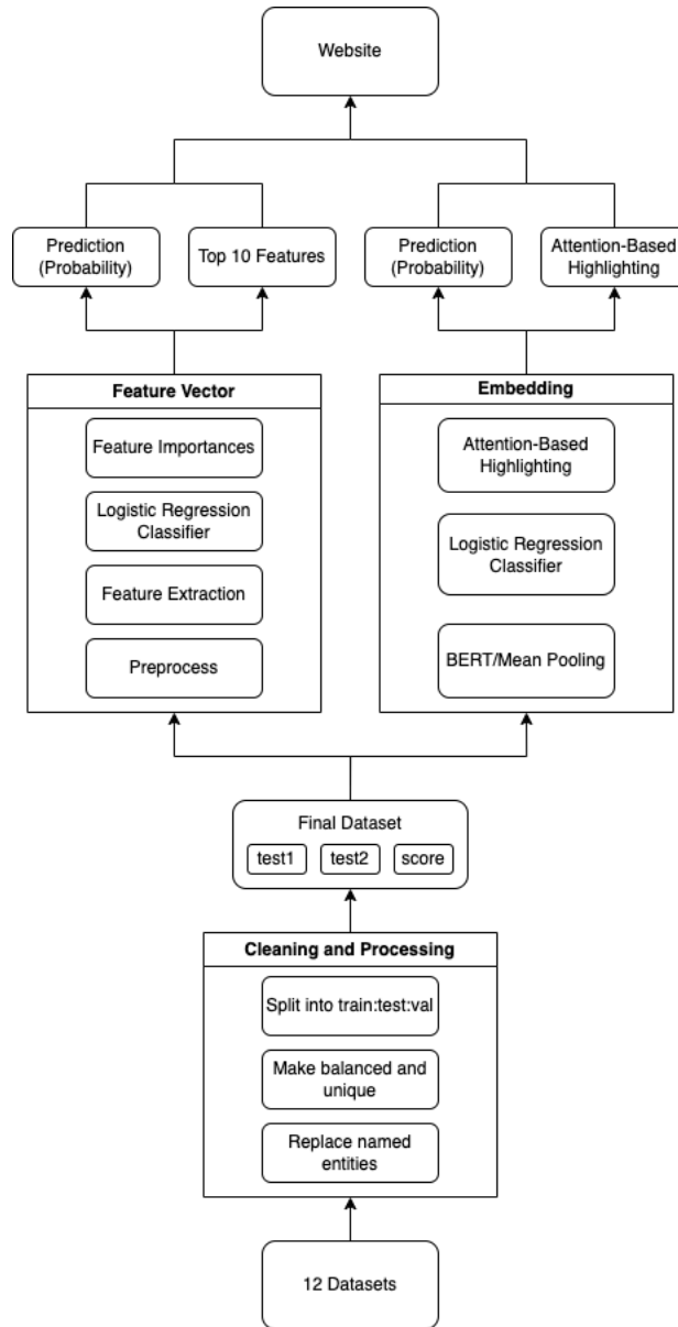
Figure 1: Overall pipeline
