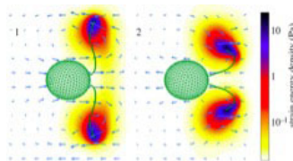
Simulations of C. reinhardtii (puller) swimming In a viscoelastic fluid showing (1) power and (2) Recovery strokes. Color bar represents polymer stresses. (Li, et al. J. Royal Soc. Interface, 2017)
