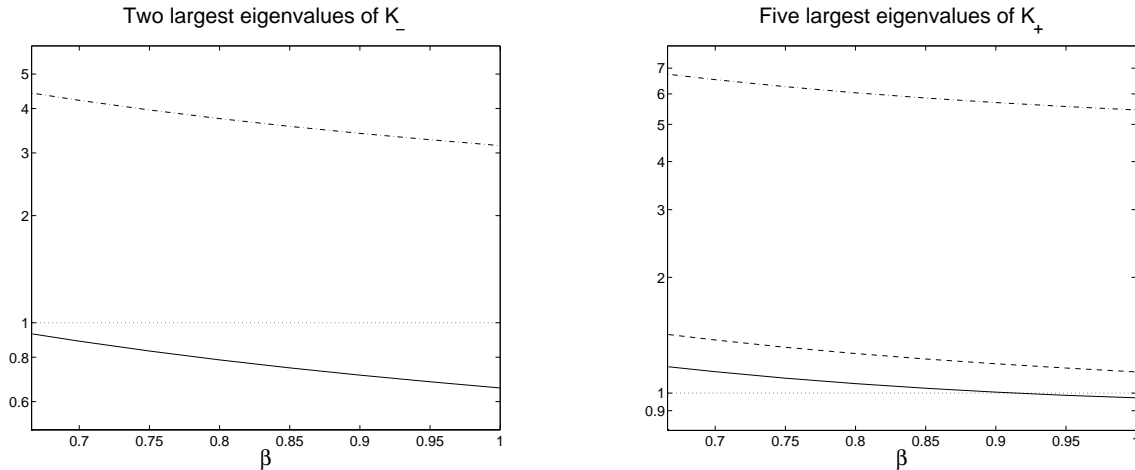
Figure 3. Left: Largest eigenvalues of K_- , as a function of \beta in the range [\frac{2}{3}, 1] . The first eigenvalue is simple, and the second to fourth are identical (multiplicity 3). Right: Five largest eigenvalues of K_+ , as a function of \beta . The first eigenvalue is simple, the second to fourth eigenvalues are identical, and the fifth eigenvalue is simple. In both cases, the value one is indicated by the dotted line.
