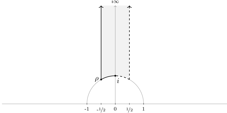
Figure 1: Fundamental domain \mathcal{F} for \mathcal{H}/\Gamma , with i = e^{\pi i/2} and \rho = e^{2\pi i/3} .
