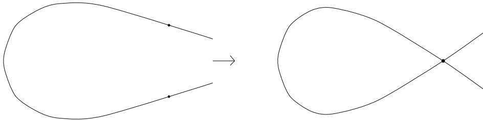
a Map to a Nodal Curve
