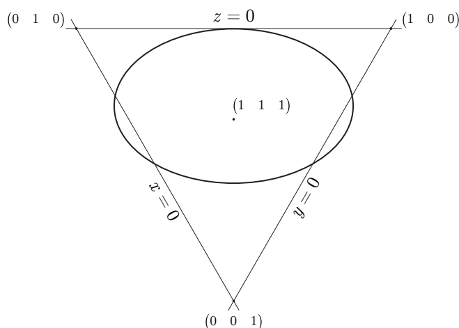
The Real Projective Plane
