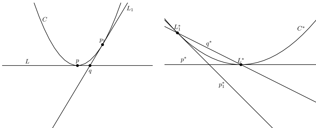
A Curve and its Dual
