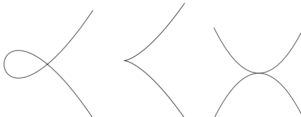
1.7.9. a Node, a Cusp, and a Tacnode (real locus)
