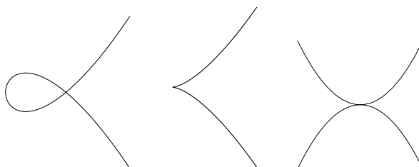
1.8.8. a Node, a Cuspidal, and a Tacnode (real locus)
