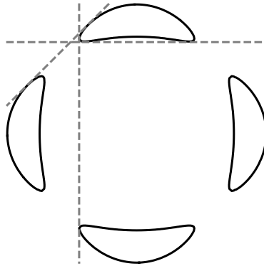
A Real Quartic Curve that has 28 Real Bitangents
