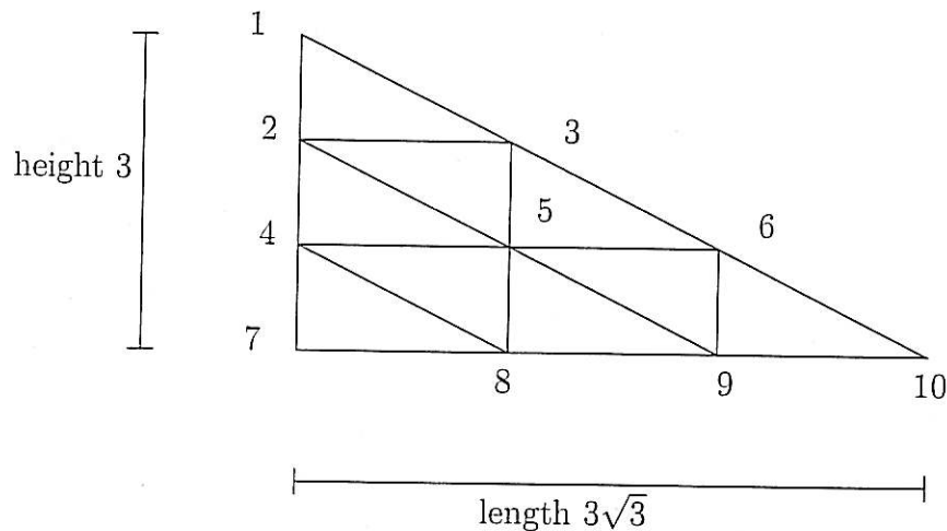
Figure 1: The triangle domain and mesh for problem 2.
