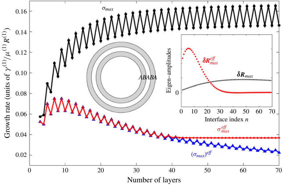
FIGURE 8. (Colour online) Growth rates of an ABABAB \dots alternating structure. Both \sigma_{max} (black line) and \sigma_{max}^{eff} (red line) converge to finite asymptotic values as N \rightarrow \infty , although in the former case the asymptotic value depends on the parity of N . The differences between \sigma_{max}^{eff} (red line) and (\sigma_{max})^{eff} (blue line) imply that the modes corresponding to \sigma_{max} and \sigma_{max}^{eff} are not always the same. The right inset shows the eigen-amplitudes \delta R_{max} (black dots) and \delta R_{max}^{eff} (red circles) for N = 70 , corresponding to \sigma_{max} and \sigma_{max}^{eff} respectively. The left inset depicts the structure whose parameters are R^{(n)} = 1 + 0.2(n - 1) , \gamma^{(n)} = 1 , and \mu^{(n)} = 1 if n is odd or \mu^{(n)} = 2 otherwise.
