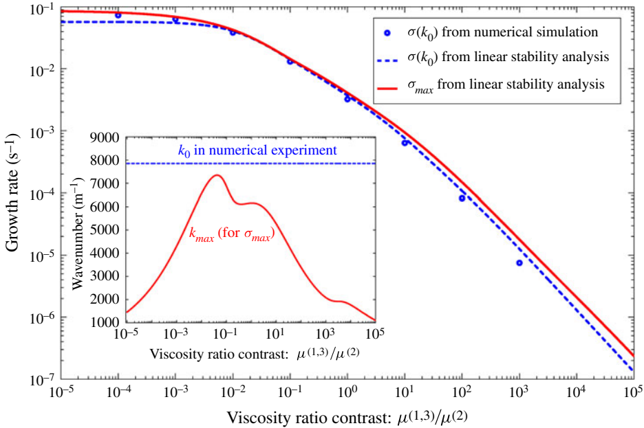
FIGURE 2. (Colour online) Comparison between linear stability analysis and numerical experiments (data from Deng et al. 2011) for N = 3 cylindrical-shell model. The growth rate \sigma_{max}(k_0) computed by Deng et al. (2011) numerically via the finite-element method (blue circles) agrees well with the growth rate predicted by linear stability analysis (dashed blue line), except for small discrepancies in the regime of large viscosity contrast where accurate numerical simulation is difficult. The red line indicates the maximum growth rate \sigma_{max} obtained by linear stability analysis. In the inset, the red line shows the wavenumbers k_{max} for various viscosity-ratio contrasts and the dashed blue line represents the fixed k_0 used in numerical simulations. Model parameters: R^{(1)} = 60 \mu\text{m} , R^{(2)} = 120 \mu\text{m} , \gamma^{(1)} = \gamma^{(2)} = 0.6 \text{ N m}^{-1} , \mu^{(2)} = 10^5 \text{ Pa s} , \mu^{(1)} = \mu^{(3)} = \eta\mu^{(2)} ( \eta = 10^{-4}, 10^{-3}, \dots, 10^3 ), and k_0 = 7.9 \times 10^3 \text{ m}^{-1} .
