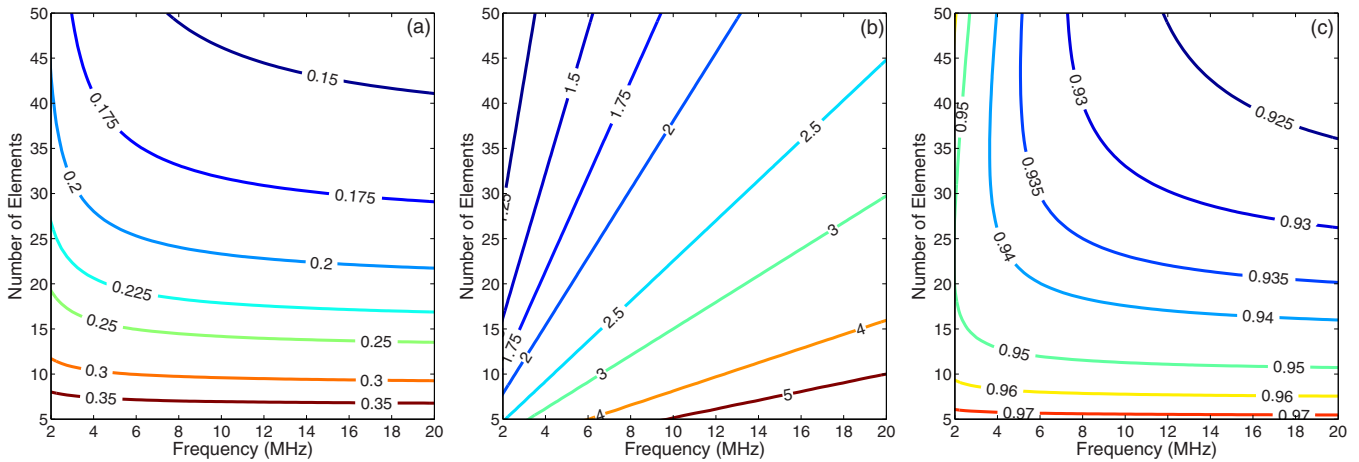
FIG. 2. (Color online) Ratio of the resistance of an optimized conducting shell structure with overall diameter 1 mm to: (a) the ac resistance of a solid conductor of the same diameter, (b) the dc resistance of the same conductor (21.6 m \Omega /m), and (c) the resistance with the same number of elements but with shells of (optimized) uniform thickness around a copper core.
