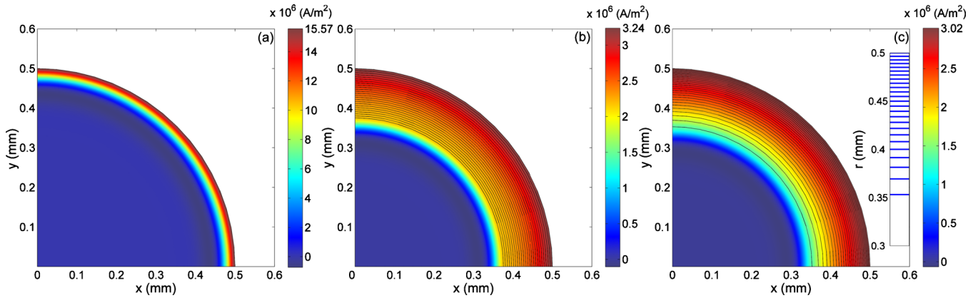
FIG. 1. (Color online) Optimal current density at 10 MHz for a copper conductor with diameter 1 mm when the wire consists of: (a) one piece of copper (resistance per length of 265.9 mΩ/m), (b) 24 mutually insulated concentric shells of equal thickness 5.19 μm around a solid copper conductor (55.2 mΩ/m), and (c) 25 elements whose thicknesses are optimized so as to minimize the overall resistance (51.6 mΩ/m). In (c), inset shows radial locations (blue) of interfaces between shells. The overall current is 1 A. For simplicity, the insulating gap between shells is taken to be negligibly small. These geometries were solved analytically in the text whereas these images were generated by a finite-element method (Ref. 9) as a check.
