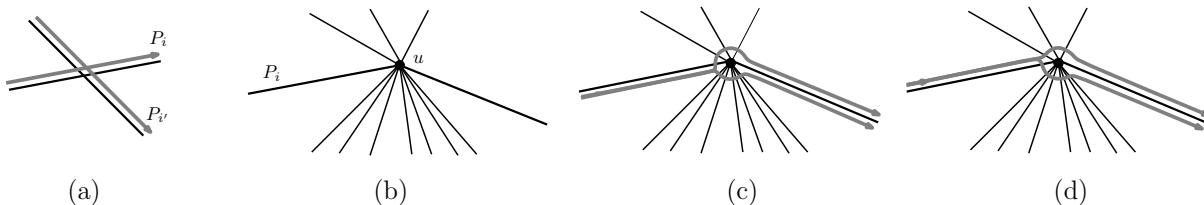
Figure 1: Drawings of edge e along two edge-disjoint path P_i and P_{i'} may give two first category crossings at a crossing of D (a). If a path P_i traverses a vertex u (b), then the edge e drawn along P_i can choose between two possible routes around u (c-d).
