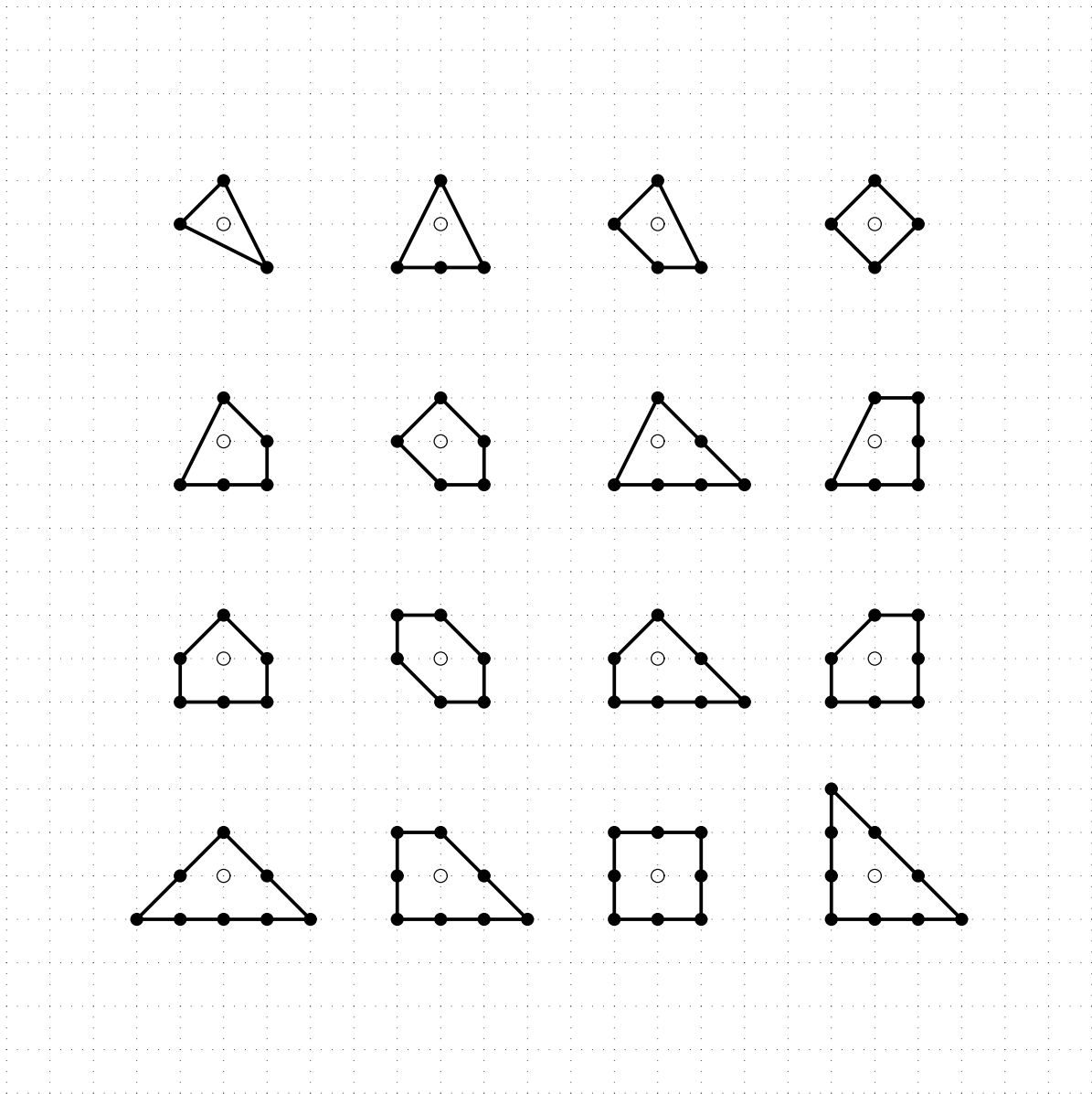
FIGURE 2. The 16 equivalence classes of legal polygons.
