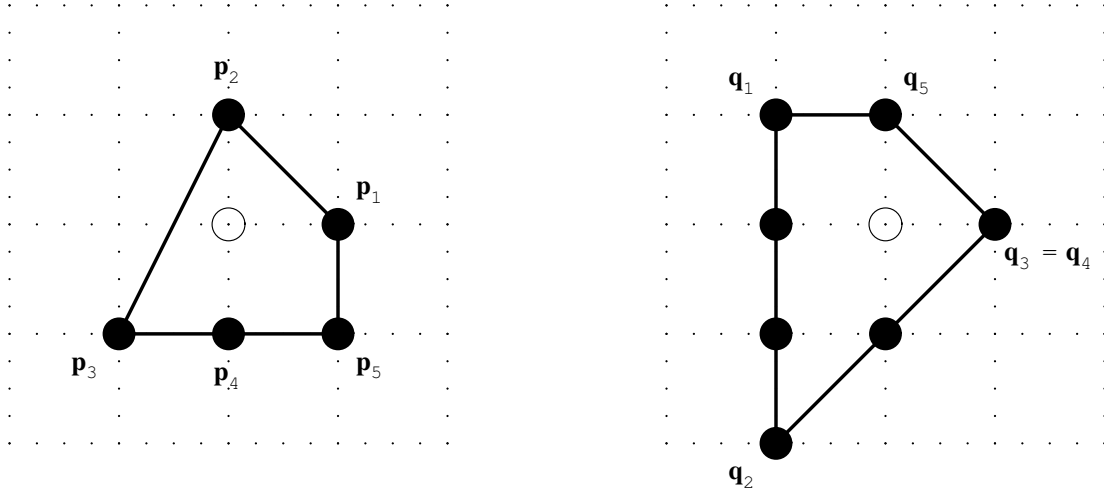
FIGURE 1. A polygon \mathcal{P} and its dual. Note that 5 + 7 = 12 .
