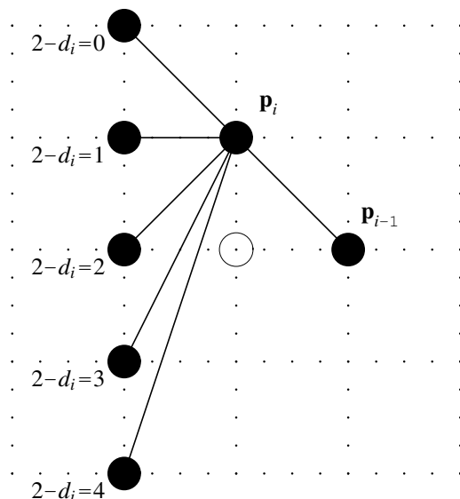
FIGURE 4. The dependence of the exterior angle at \mathbf{p}_i on 2 - d_i .
