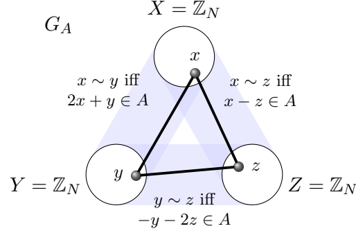
FIGURE 1. The construction in the proof of Roth's theorem.
