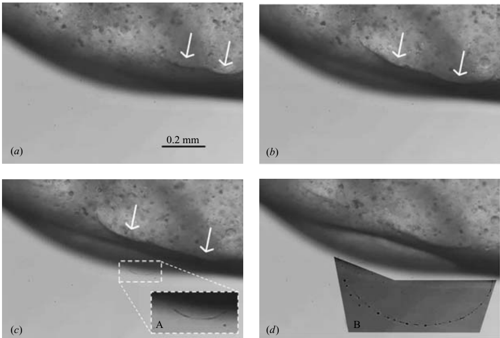
FIGURE 4. Details of an ejection event. The white arrows indicate the wave fronts moving radially outward (a, b, c) and breaking through the lens edge (c, d), ejecting oil and surfactant onto the water surface. The ejected sheet (shown in the boxed region in (c) and magnified in inset A with increased contrast), grows and breaks into droplets. The latter are evident in (d), where contrast has been enhanced in the polygonal area B to highlight the ejected material. Time between successive frames is 0.1 s.
