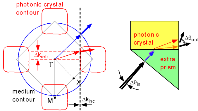
Figure 6. (Color) Left panel: dispersion-surface analysis of phase-velocity based superprism effect in our model photonic crystal, using the same notation as in Fig. 2. Right panel: illustration of a possible way of realizing this superprism effect in a prism-shaped photonic crystal (yellow), with an extra prism (green) added before the incidence interface. The thin arrows indicate the Bloch-wavevector directions inside the prisms.
