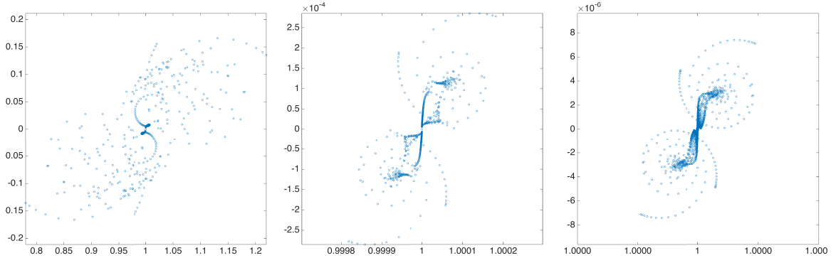
Figure 6: Eigenvalues of (\underline{\mathbf{D}})^{-1} \underline{\mathbf{P}} \underline{\mathbf{M}} , for a homogeneous media, L = 3 , n = , \omega = 30 ; and 5 ( left ), 30 ( center ) and 100 ( right ) PML points. Notice the scale of the axes.
