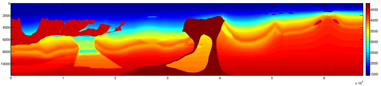
Figure 12: Geophysical benchmark model BP 2004.
