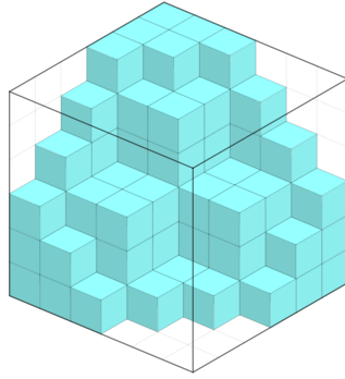
Figure 29: The center for r = 3 .
