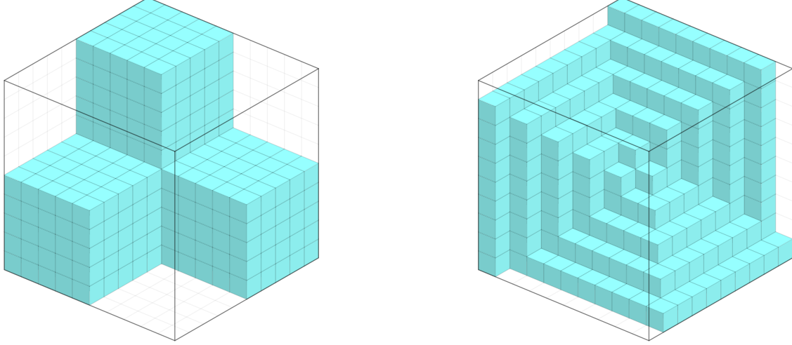
Figure 16: I and J for the case r = 5 . These ideals attain the maximum possible distance in the flip graph on cyclically symmetric self-complementary ideals of [10] \times [10] \times [10] .
