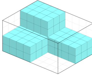
Figure 11: The unique equality case for the case (\ell_1, \ell_2, \ell_3) = (6, 8, 4) .
