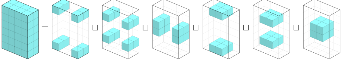
Figure 10: The partition of [2] \times [4] \times [6] into six copies of [2]^3 .
