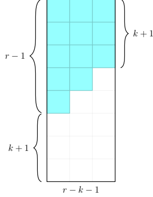
Figure 17: An example of C for the case r = 6, k = 2 .
