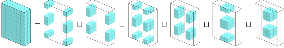
Figure 12: The partition of [2] \times [6] \times [8] into six copies of [2] \times [2] \times [4] .
