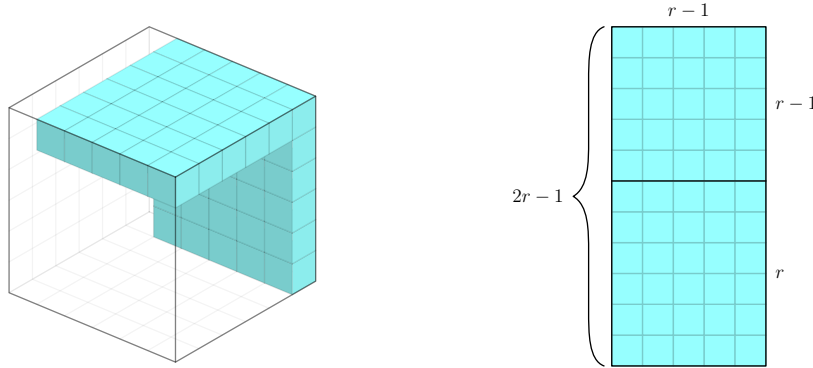
Figure 19: V \cup T for the case r = 6 is depicted on the left; note that only O_{001} is drawn. The corresponding P' is shown on the right.
