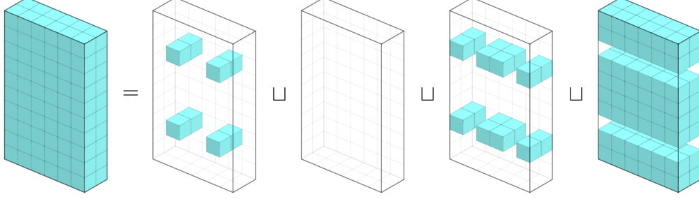
Figure 13: The partition of the poset [2] \times [6] \times [10] .
