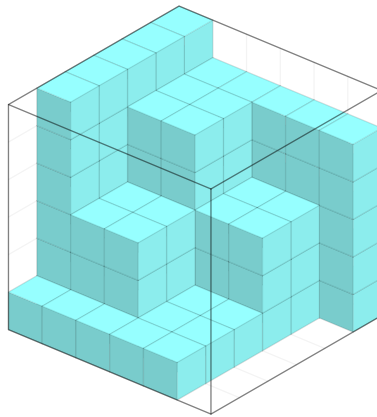
Figure 2: A cyclically symmetric self-complementary ideal of the poset [6] \times [6] \times [6] .
