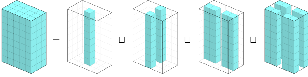
Figure 14: The partition of the poset [3] \times [5] \times [8] .
