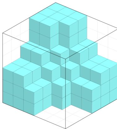
Figure 3: A totally symmetric self-complementary ideal of the poset [6] \times [6] \times [6] .
