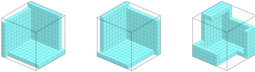
Figure 23: The three shells S_{1,10}, S_{9,10}, S_{7,10} that can surround I in Figure 22 to form an ideal in P_{10} .
