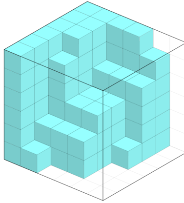
Figure 1: A self-complementary ideal of the poset [6] \times [6] \times [6] .
