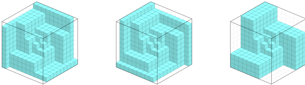
Figure 24: Three ideals in P_{10} corresponding to I in Figure 22 and the shells in Figure 23.
