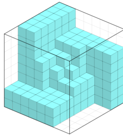
Figure 22: An example of I \in P_8 with shell S_{6,8} .
