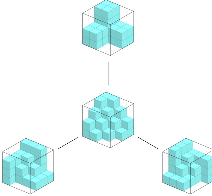
Figure 15: The flip graph on cyclically symmetric self-complementary ideals of [4] \times [4] \times [4] .
