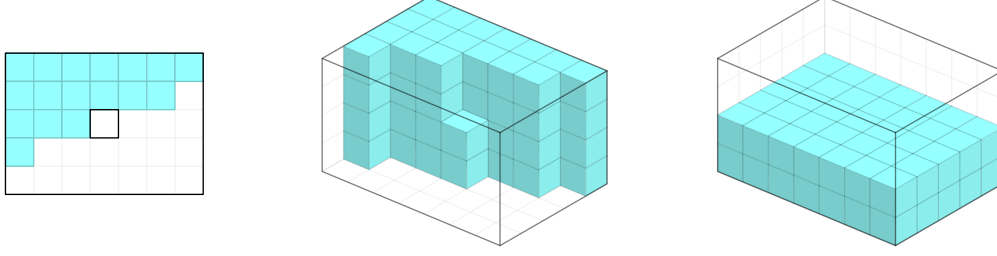
Figure 9: An example of I' , I , and J for the case (\ell_1, \ell_2, \ell_3) = (5, 7, 4) .
