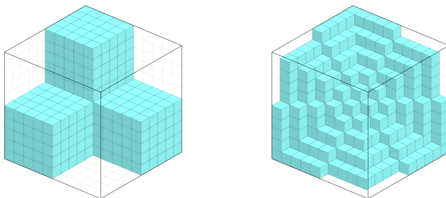
Figure 28: I and J for the case r = 5 . These ideals attain the maximum possible distance in the flip graph on totally symmetric self-complementary ideals of [10] \times [10] \times [10] .
