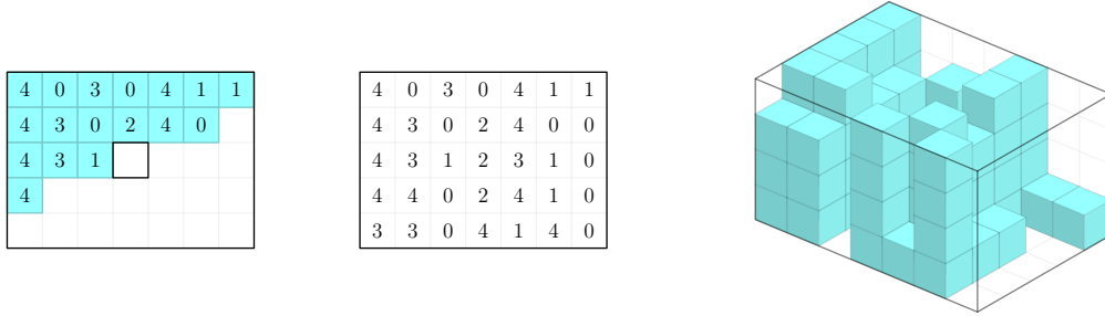
Figure 6: A sample function g : I \rightarrow \{0, \dots, n\} (that is not order-preserving) and its corresponding \tilde{g} : P \rightarrow \{0, \dots, n\} for (\ell_1, \ell_2, n) = (5, 7, 4) . The corresponding subset of [5] \times [7] \times [4] is also included.
