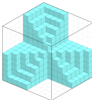
Figure 27: Points that must be included in all totally symmetric self-complementary ideals of [10] \times [10] \times [10] .
