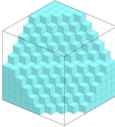
Figure 7: S for the case n = 10 , d = 3 .
