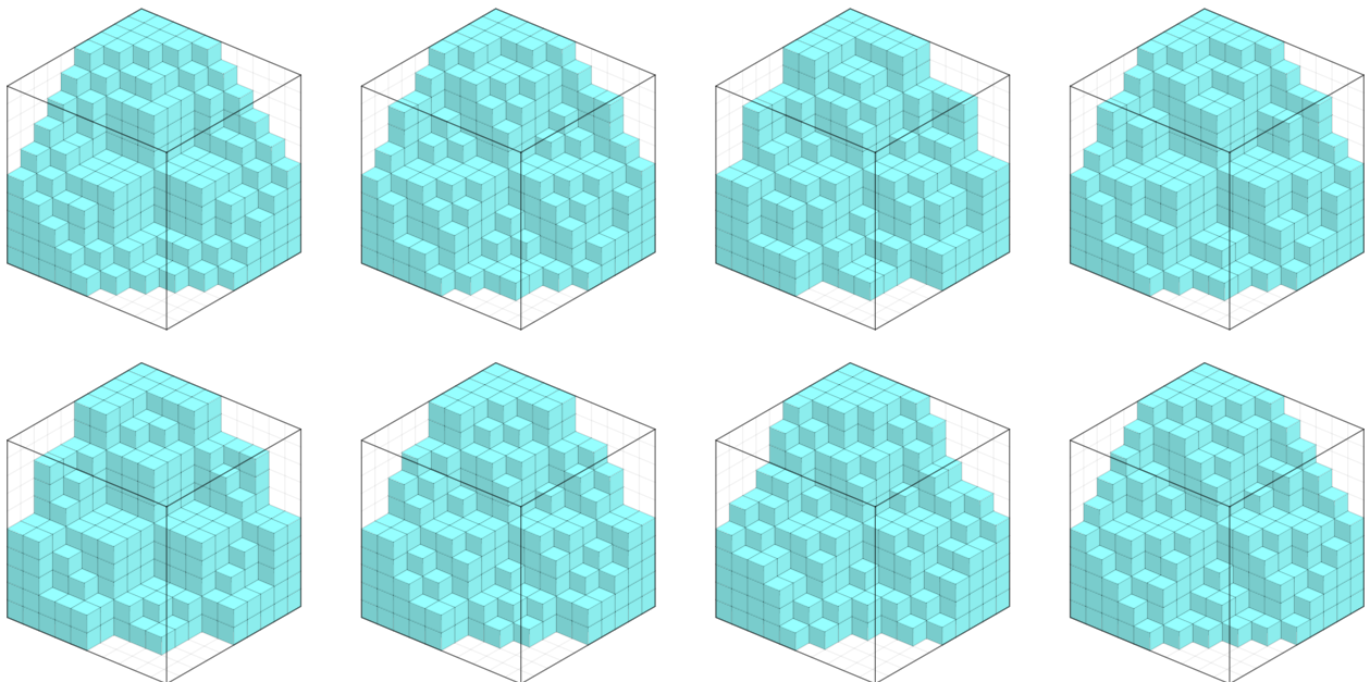
Figure 30: The center for r = 4 .
