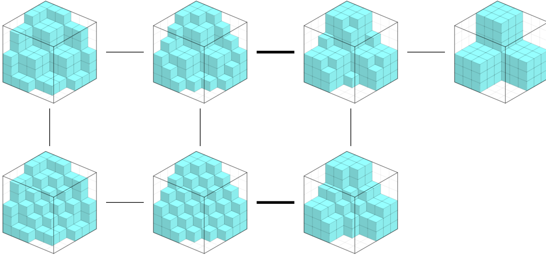
Figure 26: The flip graph on totally symmetric self-complementary ideals of [6] \times [6] \times [6] .
