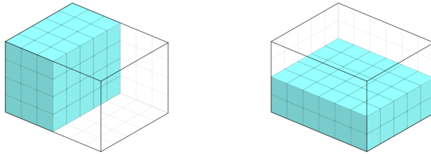
Figure 8: An example of I and J for the case (\ell_1, \ell_2, \ell_3) = (5, 6, 4) .
