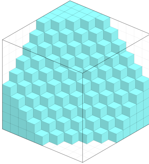
Figure 18: C_{2r} for the case r = 5 . This ideal lies in the center of the flip graph on cyclically symmetric self-complementary ideals of [10] \times [10] \times [10] .
