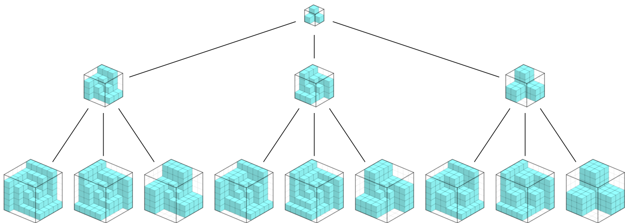
Figure 25: The first three layers of the tree structure arising from the proof of Theorem 4.3.6.
