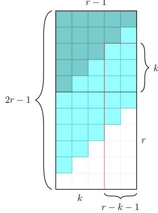
Figure 20: An example of P' for the case r = 6 , k = 3 . The highlighted cells are contained in C'_{2r} . The darker highlighted cells must also be contained in I' by Lemma 4.3.1 .
