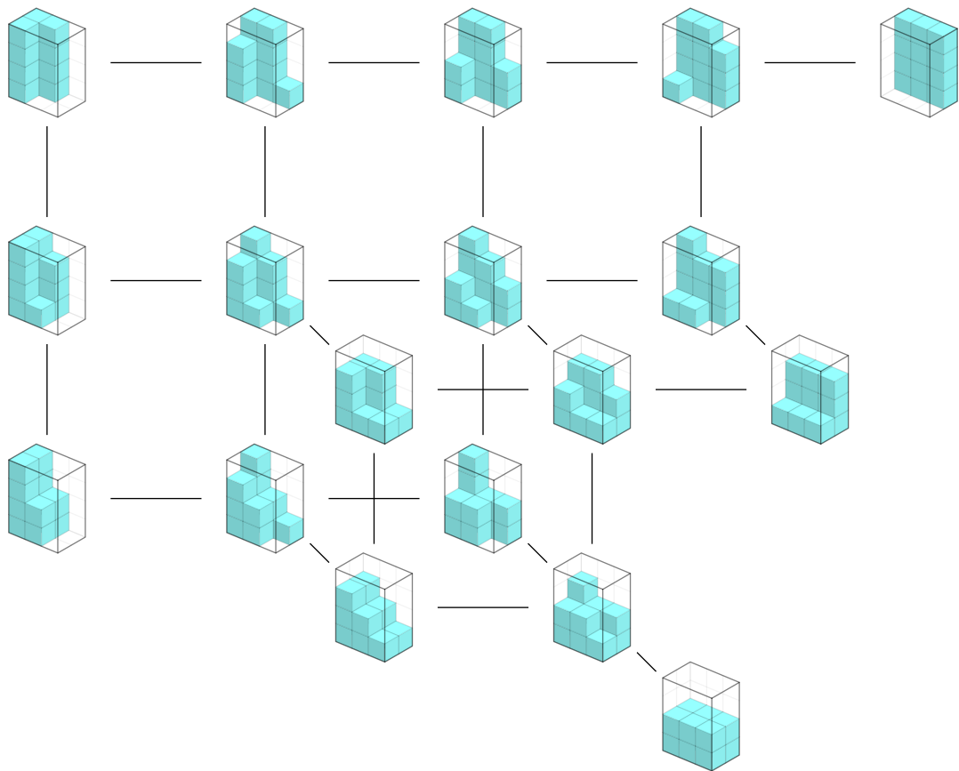
Figure 4: The flip graph on self-complementary ideals of [2] \times [3] \times [4] .
