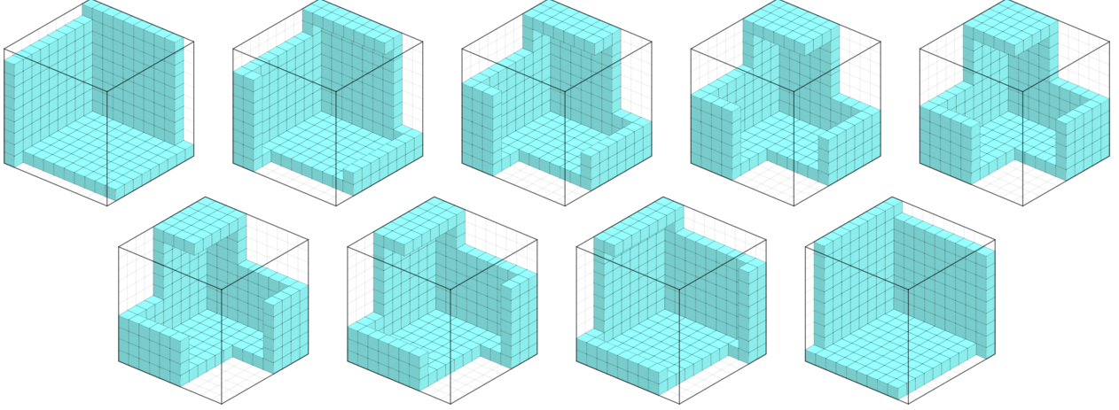
Figure 21: The shells that are equality cases for the inductive step of Lemma 4.3.4 in the case r = 5 .
