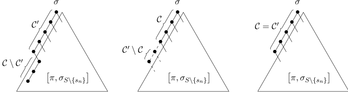
FIGURE 2. Sketches of the Hasse diagrams for the interval [\pi, \sigma] with the interval [\pi, \sigma_{S \setminus \{s_n\}}] omitted for clarity. The pertinent parts of \mathcal{C} \cup \mathcal{C}' are labeled.
