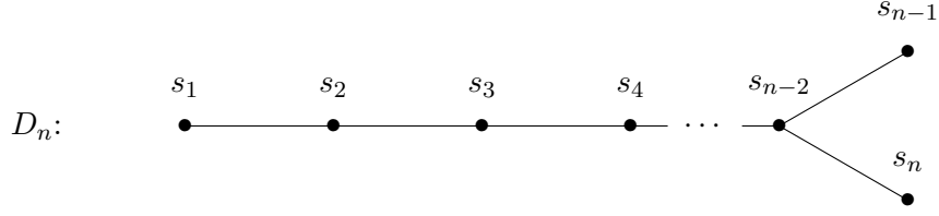
FIGURE 3. Coxeter diagram for a Coxeter system of type D_n
