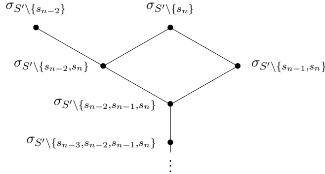
FIGURE 5. Hasse Diagram for the set [\pi, \sigma] \setminus [\pi, \sigma_{S' \setminus \{s_1\}}] , assuming no duplicates.
