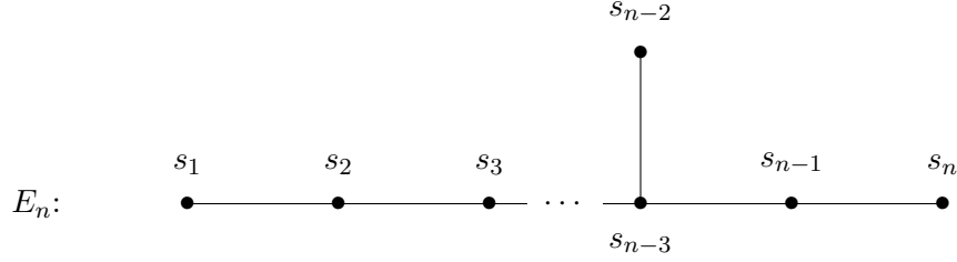
FIGURE 4. Coxeter diagram for a Coxeter system of type E_n
